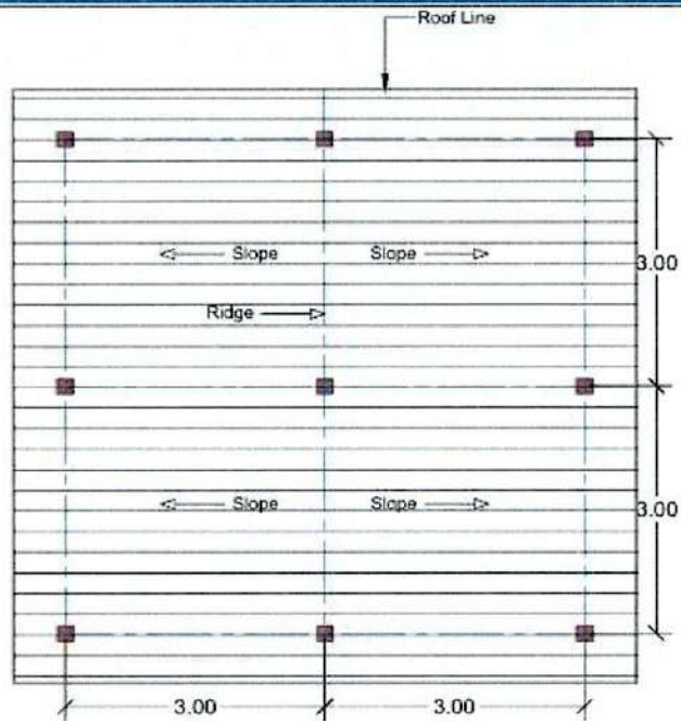
ROOF PLAN WITH CGI SHEET OR DYNA
