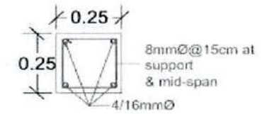
Section of All Column C1
