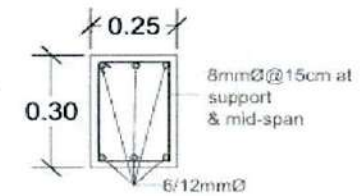
Section of Tie Beam at Ground Level
