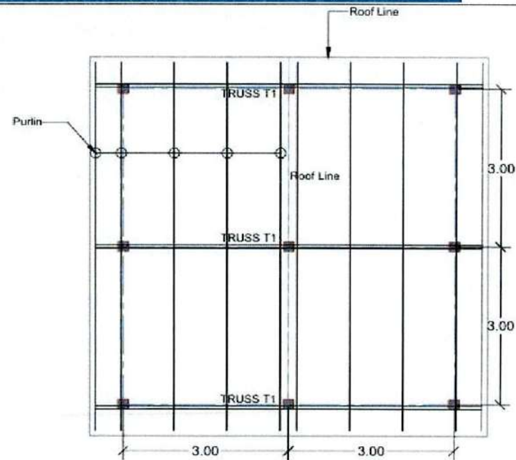
ROOF TRUSS PLAN
