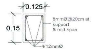
Section of Lintel at Roof Level
